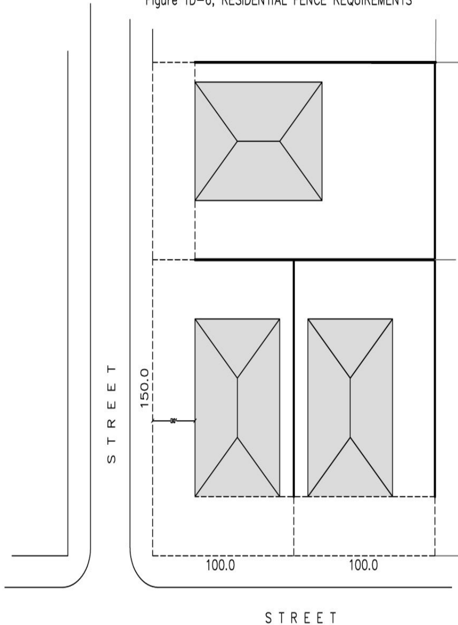
Figure 1D-6, RESIDENTIAL FENCE REQUIREMENTS
